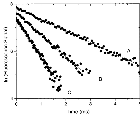
Figure 2. Typical resonance fluorescence temporal profiles observed in the study of reaction 1. Experimental conditions: T = 244 \text{ K} ; P = 15 \text{ Torr} ; [\text{NO}_2] in units of 10^{13} \text{ molecules cm}^{-3} = (\text{A}) 3.09 , (\text{B}) = 6.58 , (\text{C}) = 12.20 ; number of laser shots averaged = (\text{A}) 800 , (\text{B}) = 1000 , (\text{C}) = 2000 . Solid lines are obtained from least squares analyses and give the following first-order decay rates in units of \text{s}^{-1} : (\text{A}) 490 , (\text{B}) 940 , (\text{C}) 1620 .
