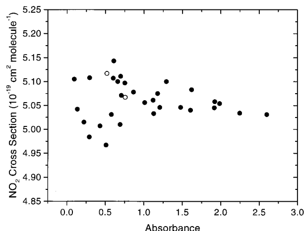
Figure 1. Plot of the calculated \text{NO}_2 absorption cross section at the argon ion laser wavelength (457.9 nm) versus absorbance. Solid circles indicate absorption cross-section measurements made with only \text{NO}_2 , while open circles indicate absorption cross-section measurements made with \text{NO}_2/\text{N}_2 mixtures at a total pressure of 100 Torr.
