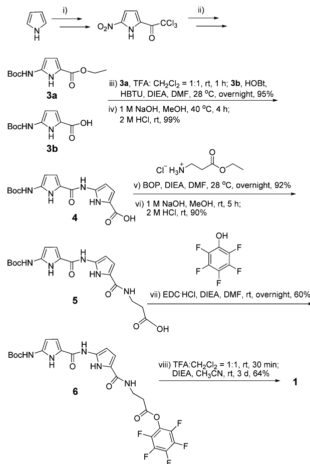
Scheme 1. Synthesis of Flexible Cyclic Polyamide 1 a
