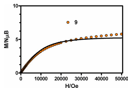
Figure 14. M vs H plot for complex 9 . The solid line corresponds to the Brillouin function for S = 5/2 .
