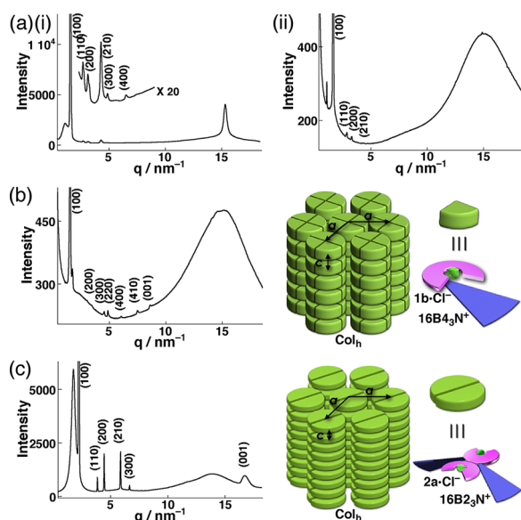
Figure 4. Representative XRD patterns of (a) 1a\text{-Cl}^-16B_{23}N^+ (i) at 25 °C after once melting to Iso and (ii) at 90 °C upon second heating, (b) 1b\text{-Cl}^-16B_{43}N^+ at 90 °C, and (c) 2a\text{-Cl}^-16B_{23}N^+ at 85 °C upon second heating. Schematic illustrations of the assembled arrangements are shown at the right in (b) and (c). Anions are shown as green spheres, anion receptors as pink partial disks, and cation modules as fanlike shapes based on the optimized structures; the charge-by-charge and charge-segregated assemblies are represented by thick and thin disk disk components, respectively.
