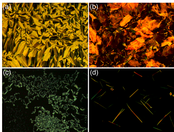
Figure 3. Representative POM textures of (a) 1a\text{-Cl}^-16B_{23}N^+ at 90 °C, (b) 1b\text{-Cl}^-16B_{43}N^+ at 125 °C, (c) 2a\text{-Cl}^-16B_{23}N^+ at 85 °C, and (d) 2b\text{-Cl}^-16B_{43}N^+ at 55 °C upon second heating after cooling from Iso.
