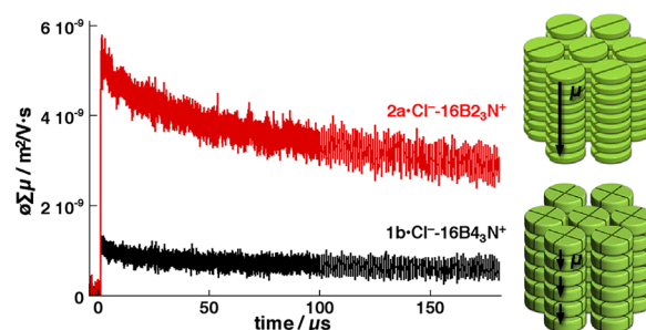
Figure 5. FP-TRMC transient signals for 1b\text{-Cl}^-16B_{43}N^+ (bottom) and 2a\text{-Cl}^-16B_{23}N^+ (top) at room temperature after once melting upon excitation at 355 nm with a power of 10 mW. Schematic illustrations of the motion of the charge carriers are shown at the right.
