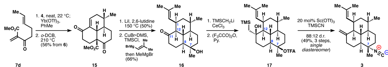
Scheme 2. Synthesis of (+)-7-Isocyano-11(20),14-epiamphilectadiene (3)
