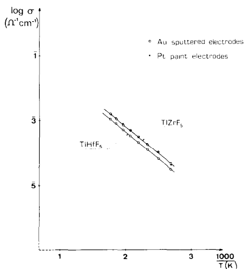
FIG. 4. Thermal variation of the ionic conductivity of both \text{TiZrF}_5 and \text{TiHfF}_5 plotted as \log \sigma versus the inverse of the absolute temperature.
