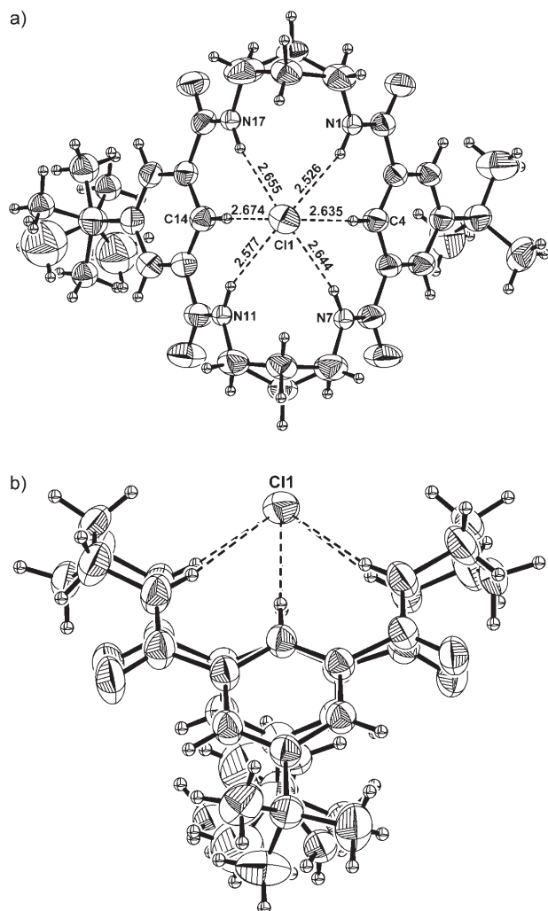
Figure 9. ORTEP view of the molecular structure of 6-Ph 4 PCl . a) Top view. b) Side view. (Part of disorder in b) has been removed for clarity. Displacement ellipsoids are scaled to the 50% probability level. Dashed lines indicate hydrogen-bonding interactions. The distances are given in angstroms.)
