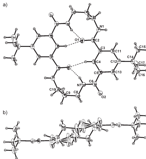
Figure 6. ORTEP view of the molecular structure of 6 ·CH 3 OH. a) Top view, atom numbering is limited to symmetrically independent part. b) Side view. (Displacement ellipsoids are scaled to the 30% probability level. Dashed lines indicate hydrogen-bonding interactions.)
