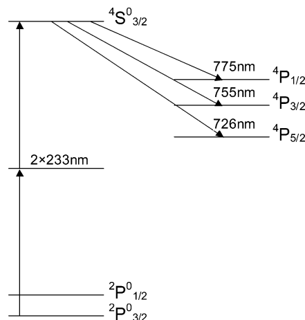
Figure 3. Excitation scheme for the two-photon LIF of Cl atoms. The excitation transition is at 2 \times 233 \text{ nm} with the subsequent fluorescence transition near 755 nm.
