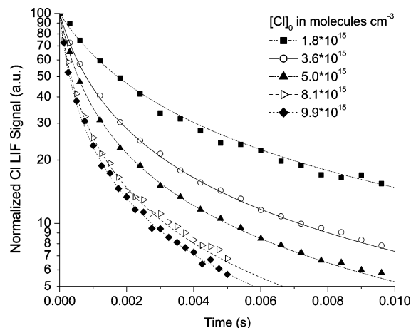
Figure 4. Typical chlorine atom temporal profiles, shown for measurements conducted in 600 Torr N 2 at 293 K.
