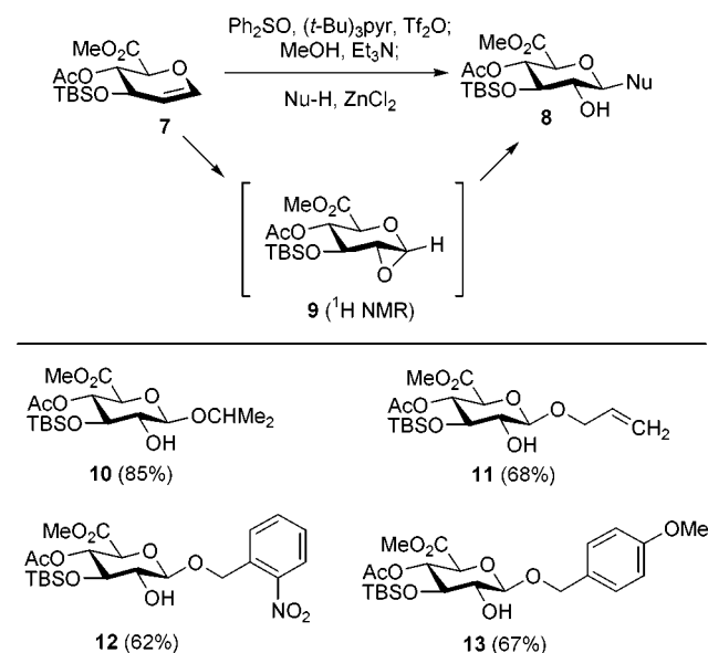
Figure 1. Oxidative glycosylation with glycol 7 .
