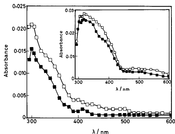
Figure 3. Transient absorption spectra recorded in \text{N}_2 -saturated solutions ( \text{pH} = 10 ) of caffeine ( 1 \times 10^{-3} \text{ M} ) containing \text{K}_2\text{S}_2\text{O}_8 ( 1.5 \times 10^{-2} \text{ M} ) and 0.2 M tert -butyl alcohol at 18 \mu\text{s} (□) after the pulse and in \text{N}_2\text{O}-\text{O}_2 (4:1 v/v) saturated neutral solutions at 7 \mu\text{s} (■) after the pulse. This spectrum is normalized to a G value of 3.3. Inset: Transient absorption spectra recorded for the reaction of \text{SO}_4^{\cdot-} at neutral pH at 2 (□) and 18 \mu\text{s} (■) after the pulse. Dose:pulse = 15 Gy.
