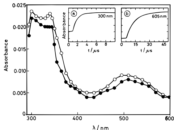
Figure 4. Absorption spectra for \text{O}^{\cdot-} reaction recorded in \text{N}_2\text{O} -saturated basic solutions ( \text{pH} \geq 13 ) of caffeine ( 1 \times 10^{-3} \text{ M} ) at 2 (○) and 18 \mu\text{s} (●) after the pulse. Dose:pulse = 15 Gy. Inset: (a) Buildup at 300 nm and (b) the rate of formation of \text{MV}^{\cdot+} at 605 nm. Dose: pulse = 12 Gy.
