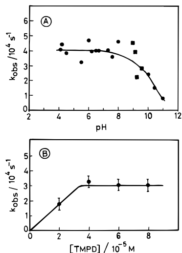
Figure 2. (A) Dependence of the rate constants for the decay at 500 nm (●) and \text{OH}^- elimination (■) from conductance measurements on pH. (B) Dependence of the rate ( k_{\text{obs}} ) of increase in absorption at 610 nm (●) on [\text{TMPD}] . For both (A) and (B), [\text{caffeine}] = 1 \times 10^{-3} \text{ M} .
