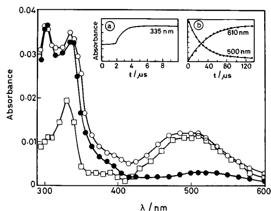
Figure 1. Transient absorption spectra measured in \text{N}_2\text{O} saturated neutral solutions of caffeine ( 1 \times 10^{-3} M) at 2 (○) and 20 \mu\text{s} (●) after the pulse. (□) This plot is drawn from the difference in the fully grown spectra recorded in the absence and the presence of \text{O}_2 at 7 \mu\text{s} . Dose/pulse = 15 Gy. Inset: Traces showing the (a) buildup at 335 nm [caffeine] = 4 \times 10^{-4} M and (b) first-order decay at 500 nm and the corresponding growth of \text{TMPD}^{\bullet+} at 610 nm on pulsing \text{N}_2\text{O} -saturated neutral solutions [caffeine] = 1 \times 10^{-3} M. Dose/pulse was 12 Gy.
