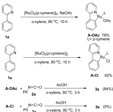
Scheme 2. Structure and Reactivity of Intermediate A
