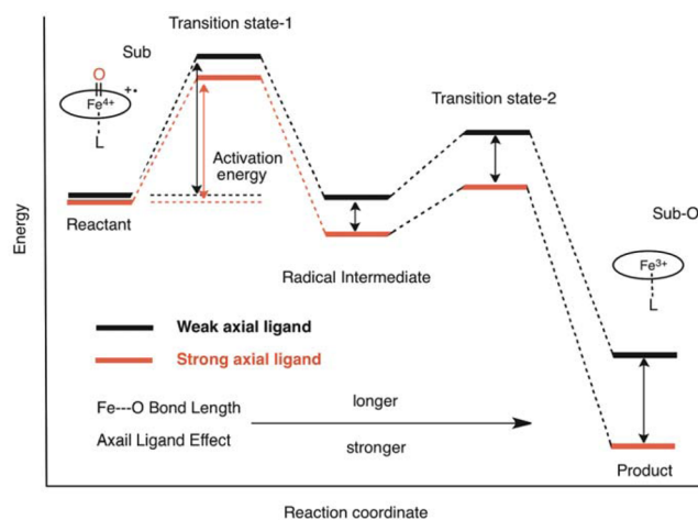
Figure 8. Cartoon of the axial ligand effect on energy profiles along the reaction of (TMP + •)Fe IV O(L) with a substrate in a stepwise mechanism. The black lines are the cases for the weak binding axial ligand and the red line is that for strong ones.
