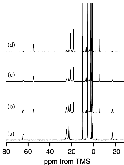
Figure 3. 1 H NMR spectral change for the titration of (TMP + •)-Fe IV O(NO 3 ) with n -Bu 4 N(Cl) in CD 2 Cl 2 at -60 °C. (a) (TMP + •)-Fe IV O(NO 3 ), (b) (a) + 0.5 equiv of n -Bu 4 N(Cl), (c) (a) + 1.0 equiv of n -Bu 4 N(Cl), (d) (a) + 1.5 equiv of n -Bu 4 N(Cl).
