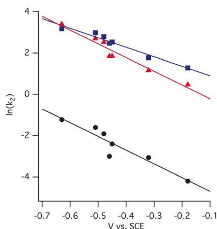
Figure 2. Plot of \ln of the reaction rate constants ( k_2 ) of the reaction of (TMP + •)Fe IV O(L) with cyclooctene (black circle), N,N -dimethyl- p -nitroaniline (red triangle), and 1,4-cyclohexadiene (blue square) vs the redox potential for Fe II /Fe III redox process of (TMP)Fe III (L).
