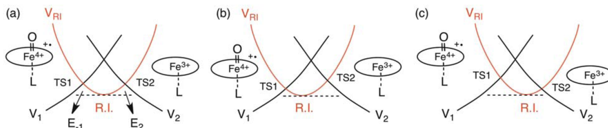
Figure 9. Curve crossing diagram of potential-energy surfaces from (\text{TMP}^{\bullet})\text{Fe}^{\text{IV}}\text{O}(\text{L}) to (\text{TMP})\text{Fe}^{\text{III}}(\text{L}) for a stepwise mechanism. V_1 and V_2 indicate the potential curves of (\text{TMP}^{\bullet})\text{Fe}^{\text{IV}}\text{O}(\text{L}) and (\text{TMP})\text{Fe}^{\text{III}}(\text{L}) , respectively. V_{\text{RI}} shows the potential curve of a radical intermediate (R.I.). E_{-1} is the activation energy from R.I. to (\text{TMP}^{\bullet})\text{Fe}^{\text{IV}}\text{O}(\text{L}) and E_2 is the activation energy from R.I. to (\text{TMP})\text{Fe}^{\text{III}}(\text{L}) . (a) E_1 \approx E_2 , (b) E_1 < E_2 , and (c) E_1 \gg E_2 .
