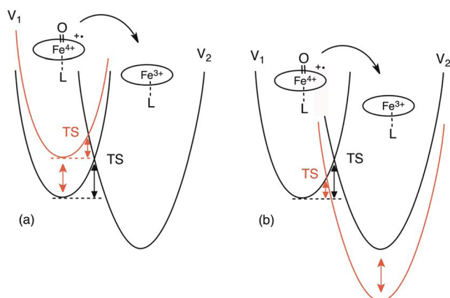
Figure 7. Curve crossing diagram of potential-energy surfaces of the reactant, (TMP + •)Fe IV O(L), and product, (TMP)Fe III (L), states. V 1 and V 2 indicate the potential curves of (TMP + •)Fe IV O(L) and (TMP)Fe III (L), respectively. TS is the transition state of the reaction. (a) Change of stability of (TMP + •)Fe IV O(L) and (b) change of stability of (TMP)Fe III (L).
