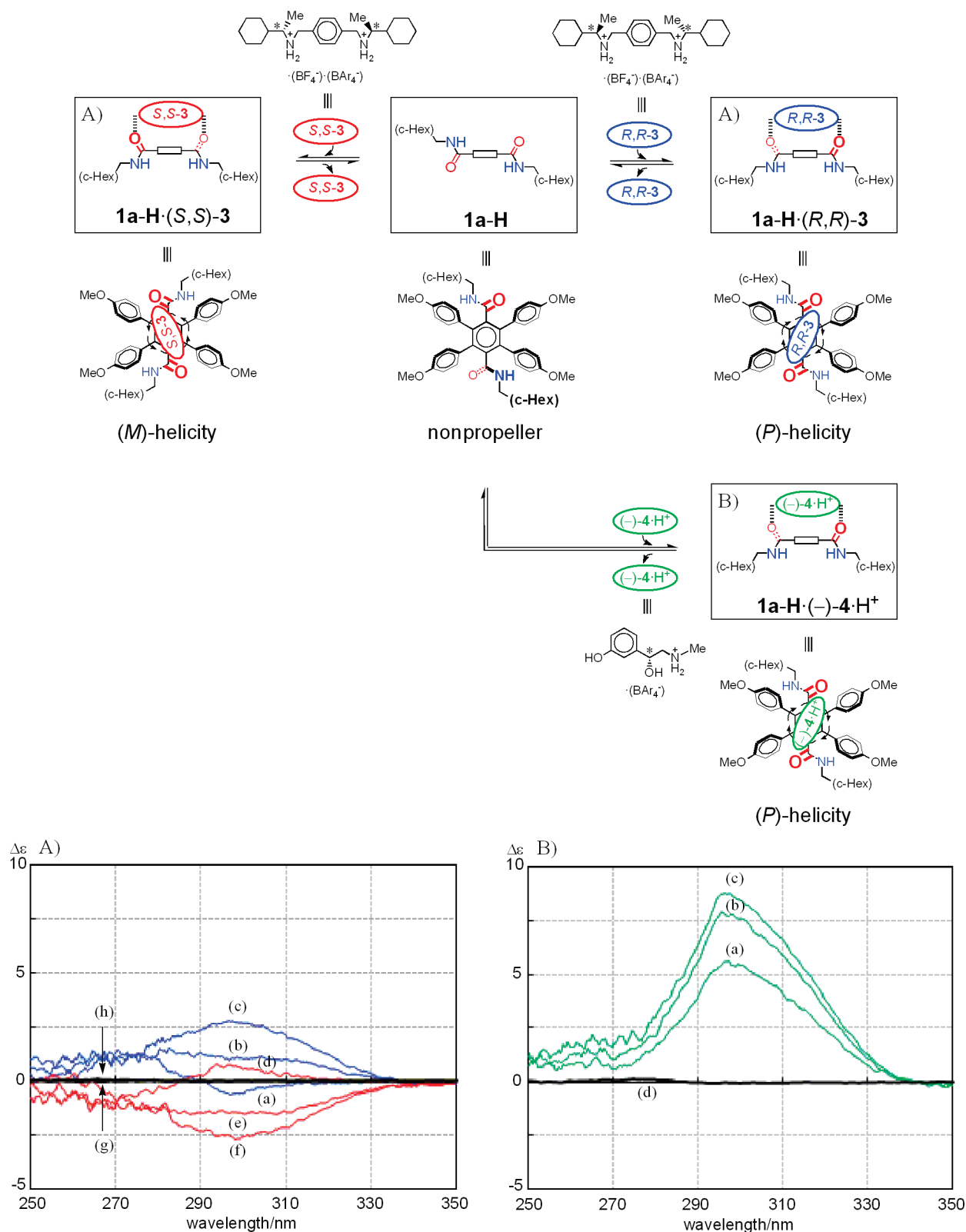
Figure 4. (A) Continuous changes in the CD spectrum upon complexation of achiral host 1a-H ( 4.2 \times 10^{-4} M) with ( R,R )/( S,S )- 3 ; (a) 1 equiv. ( 4.2 \times 10^{-4} M), (b) 2 equiv. ( 8.3 \times 10^{-4} M), (c) 4 equiv. ( 1.7 \times 10^{-3} M) of ( R,R )- 3 (blue line), (d) 1 equiv. ( 4.2 \times 10^{-4} M), (e) 2 equiv. ( 8.3 \times 10^{-4} M), (f) 4 equiv. ( 1.7 \times 10^{-3} M) of ( S,S )- 3 (red line), and CD spectra of (g) ( R,R )- 3 (black line; 2.7 \times 10^{-4} M), and (h) ( S,S )- 3 (black line; 2.5 \times 10^{-4} M); (B) Continuous changes in the CD spectrum upon complexation of 1a-H ( 2.8 \times 10^{-4} M) with (–)-phenylephrine 4 ·HBAr 4 ; (a) 1 equiv. ( 2.8 \times 10^{-4} M), (b) 2 equiv. ( 5.5 \times 10^{-4} M), (c) 4 equiv. ( 1.1 \times 10^{-3} M) (green line), and (d) CD spectrum of 4 ·HBAr 4 (black line; 1.8 \times 10^{-4} M). All spectra were measured in \text{CH}_2\text{Cl}_2 at room temperature.
