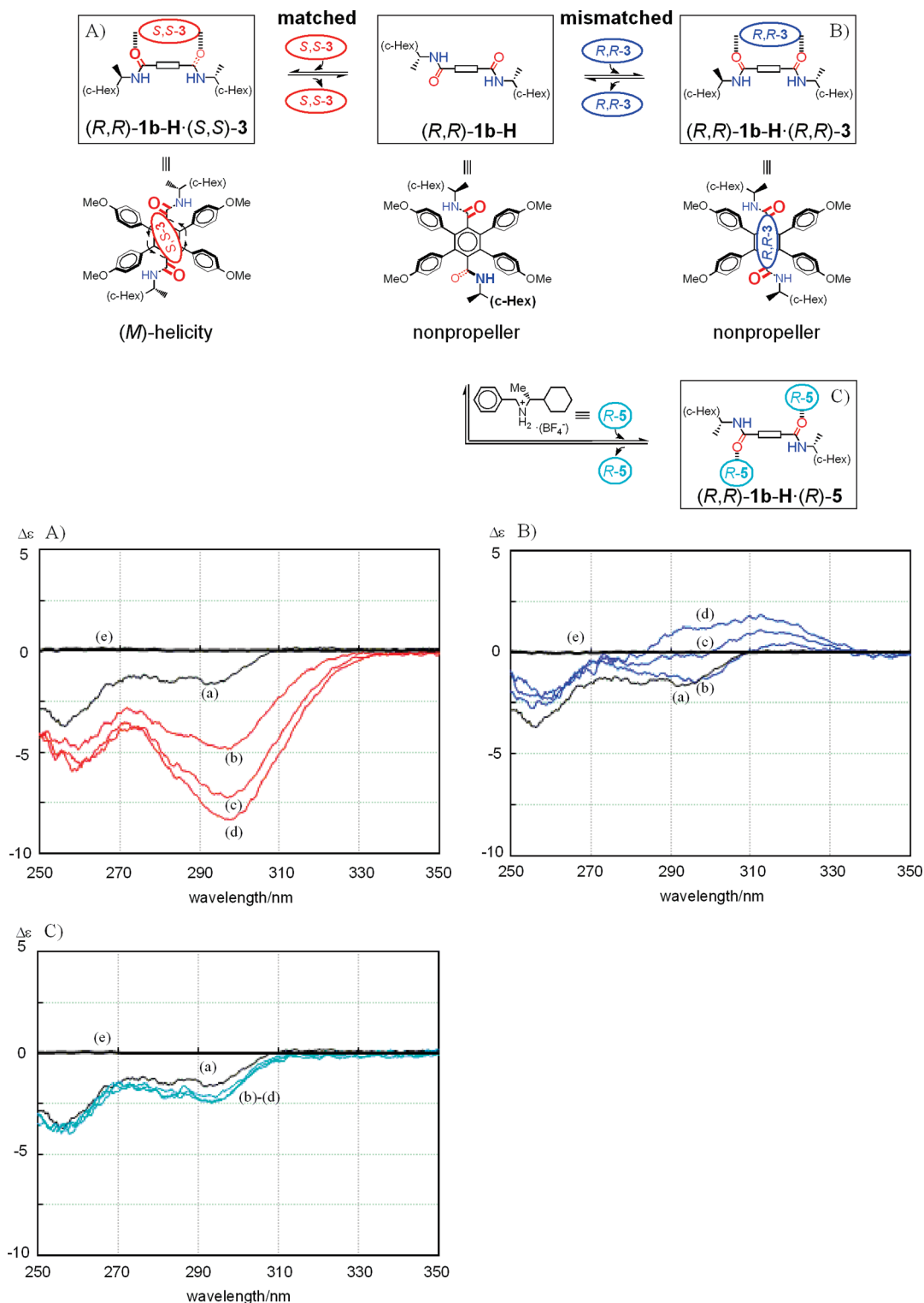
Figure 7. (A) Continuous changes in the CD spectrum upon complexation of chiral host (R,R) -1b-H ( 3.0 \times 10^{-4} M) with (S,S)-3; (a) 0 equiv. ( (R,R) -1b-H only (thin black line)), (b) 1 equiv. ( 3.0 \times 10^{-4} M), (c) 2 equiv. ( 6.0 \times 10^{-4} M), (d) 4 equiv. ( 1.2 \times 10^{-3} M) (red line), and (e) CD spectrum of (S,S)-3 (bold black line; 2.5 \times 10^{-4} M); (B) Continuous changes in the CD spectrum upon complexation of (R,R) -1b-H ( 3.0 \times 10^{-4} M) with (R,R)-3; (a) 0 equiv. ( (R,R) -1b-H only (thin black line)), (b) 1 equiv. ( 3.0 \times 10^{-4} M), (c) 2 equiv. ( 6.0 \times 10^{-4} M), (d) 4 equiv. ( 1.2 \times 10^{-3} M) (blue line), and (e) CD spectrum of (R,R)-3 (bold black line; 2.7 \times 10^{-4} M); (C) Continuous changes in the CD spectrum upon complexation of (R,R) -1b-H ( 3.2 \times 10^{-4} M) with (R)-5; (a) 0 equiv. ( (R,R) -1b-H only (thin black line)), (b) 1 equiv. ( 3.2 \times 10^{-4} M), (c) 2 equiv. ( 6.5 \times 10^{-4} M), (d) 4 equiv. ( 1.3 \times 10^{-3} M) (sky blue line), and (e) CD spectrum of (R)-5 (bold black line; 3.5 \times 10^{-3} M). All spectra were measured in \text{CH}_2\text{Cl}_2 at room temperature.
