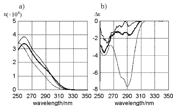
Figure 2. (a) UV and (b) CD spectra of ( R,R )- 1b-H (bold line), anti -( R,R )- 1b-Me (thin line), and syn -( R,R )- 1b-Me (dashed line) measured in CH 2 Cl 2 at room temperature.
