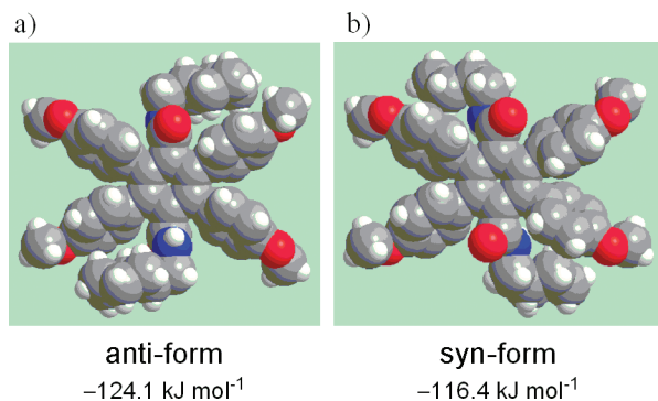
Figure 1. Energy-minimized structures of 1a-H adopting (a) anti-form (achiral nonpropeller geometry) and (b) syn-form (chiral propeller geometry) according to Monte Carlo simulations in CHCl 3 . The anti-form preference over syn-forms is also the case for the N,N' -dimethyl derivative (anti: -108.0 kJ mol -1 ; syn: -104.9 kJ mol -1 ) where the methyl groups are replaced for the cyclohexylmethyl groups, thus the bulkiness of cyclohexyl group does nothing to do with the anti-preference in 1a-H .
