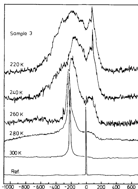
FIG. 1. ^{19}\text{F} NMR spectra of sample 3 at different temperatures.
