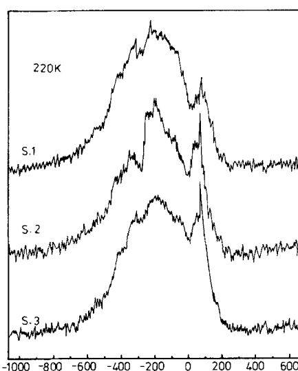
FIG. 2. Low temperature (220 K) ^{19}\text{F} NMR spectra of three compounds. (1) F/Nb = 5.96; (2) F/Nb = 5.79; (3) F/Nb = 5.67.
