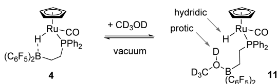
Scheme 5. Reversible Adduct Formation with Methanol and Activation for H/D Exchange
