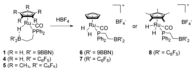
Scheme 3. Protonation of Complexes 1, 4, and 5 To Give Cationic Dihydrogen Complexes 6 and 7 or Dihydride 8
