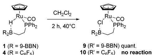
Scheme 4. Reactivity towards Chlorinated Hydrocarbons
