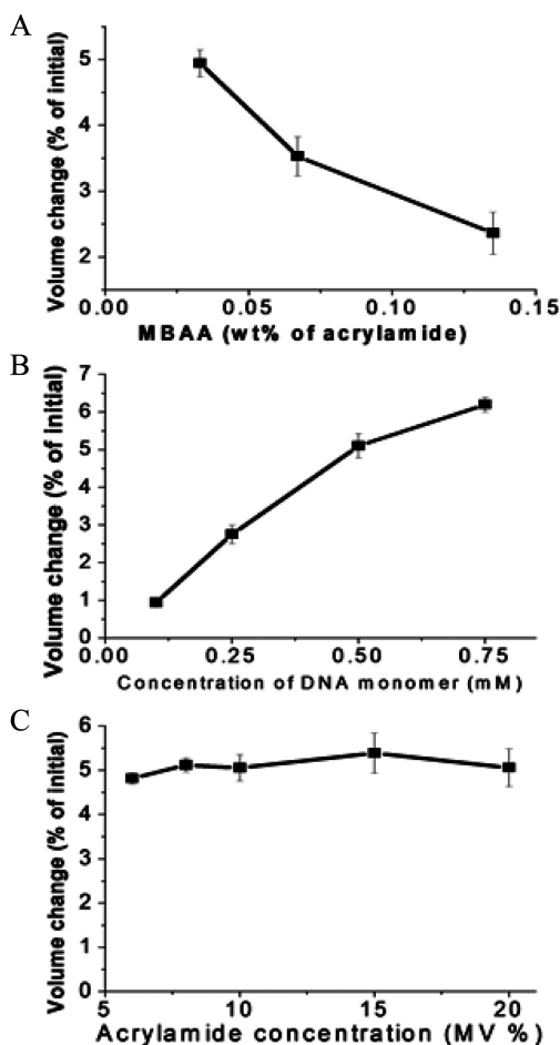
Figure 5. Percentage reversible volume change of light-responsive dynamic hydrogels synthesized under different conditions: (A) percentage volume change as a function MBAA concentration; (B) percentage volume change as a function of DNA monomer concentration; (C) percentage volume change as a function of acrylamide concentration.
