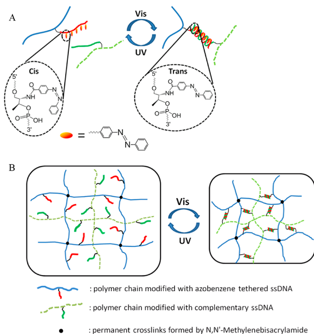
Figure 1. (A) Light-controlled formation of DNA duplex based on azobenzene isomerization in the hydrogel. (B) Reversible volume transition of the DNA-cross-linked hydrogel regulated by UV and visible light.
