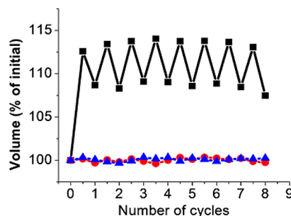
Figure 4. Reversible swelling and shrinking of light-responsive dynamic hydrogels in response to alternate irradiation by UV and visible light. Black curve: dynamic hydrogel containing cDNAs with azobenzene modification. Blue curve: control hydrogel (C1) containing cDNAs without azobenzene modification. Red curve: control hydrogel (C2) containing noncDNAs with azobenzene modification.
