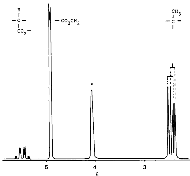
Figure 3 —Part spectrum of I treated with 0.28 equivalent of tris-(3-heptafluorobutyl-d-camphorato)europium. Starred peak is due to europium reagent.
