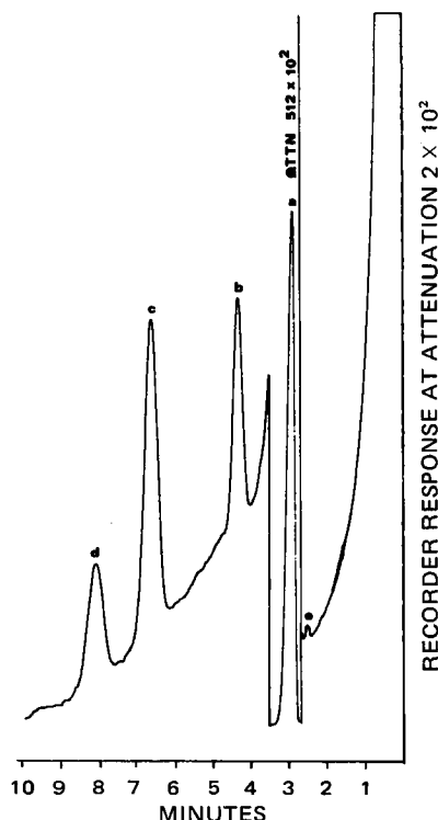
Figure 1 —Gas chromatogram from a sample containing 0.5% of VI and VII in I. Key: a, main component, methyl 4-chlorobenzoate; b, methyl 3-chlorobenzoate; c, internal standard, 4-chloroacetophenone; d, methyl 2-chlorobenzoate; and e, peak present in blank. The conditions were: 5% IX–4% diisooctyl phthalate on 80–100-mesh Gas Chrom Q, nitrogen flow rate of 30 ml/min, and column temperature of 180°.
