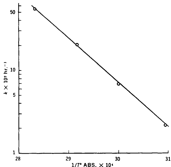
Figure 3—Typical Arrhenius plot for observed first-order velocity constants related to decomposition of 5-diethylaminodibenzo[a,d]cycloheptane (Table I, Compound I) in 0.1 N HCl at various temperatures.
