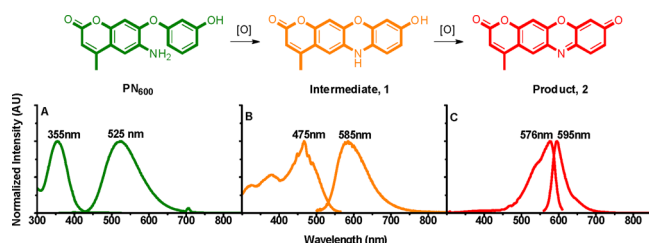
Figure 1. Detection scheme and normalized excitation/emission spectra of (A) PN 600 , (B) 1, and (C) 2. The \epsilon \times \phi of PN 600 , 1, and 2 were found to be 9000 \times 0.09 in H 2 O, 17\,000 \times 0.01 in H 2 O, and 31\,000 \times 0.62 in EtOH, respectively. The values of \epsilon are given in units of \text{cm}^{-1} \text{M}^{-1} .
