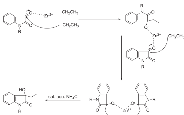
Scheme 2. The reaction between Et 2 Zn and N-substituted isatin.
