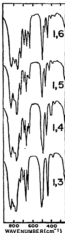
Fig. 5. IR spectra for \alpha,\omega -dichloropolysilanes (CsI, thin film).
