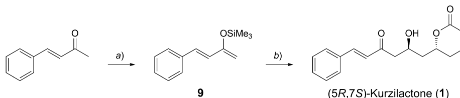
Scheme 3. Synthesis of (5 R ,7 S )-Kurzilactone ( 1 )
