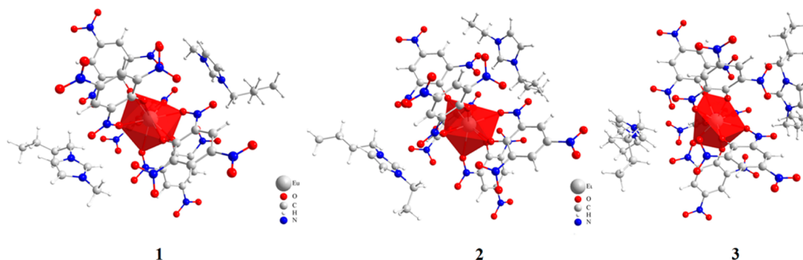
Figure 3. Calculated ground-state geometries, using the Sparkle/PM3 model, for complexes 1 , 2 , and 3 .
