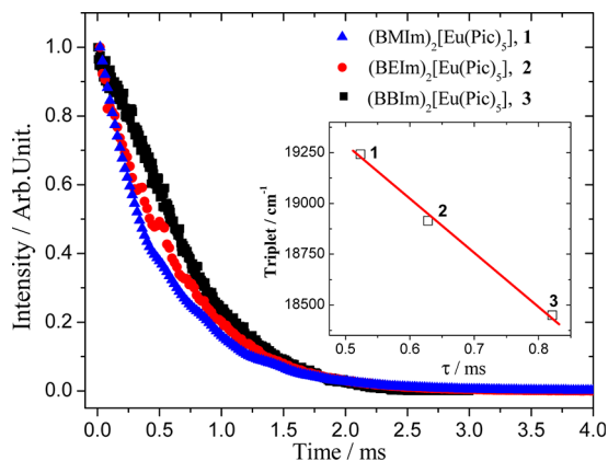
Figure 9. Decay luminescence curves of complexes 1 , 2 , and 3 recorded at 77 K monitored with excitation at 370 nm and emission at 616 nm. The inset shows the relation between the lifetimes of the ^5D_0 level and the T_1 position.
