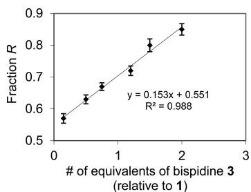
Figure 1. Resolution of 2 by 4 with varying amounts of bispidine 3 (0 ^\circ\text{C} , 1 h). 9
