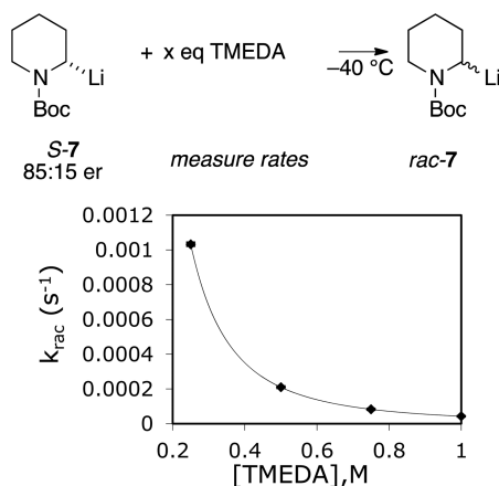
Figure 13. Effect of 1–4 equiv of TMEDA on the rate of racemization of 7 (0.25 M) at -40\text{ }^\circ\text{C} .
