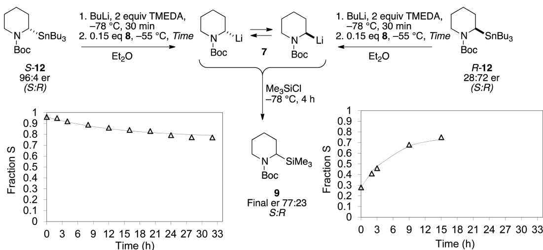
Figure 14. Evolution of CDR starting from enantioenriched R - or S -12.
