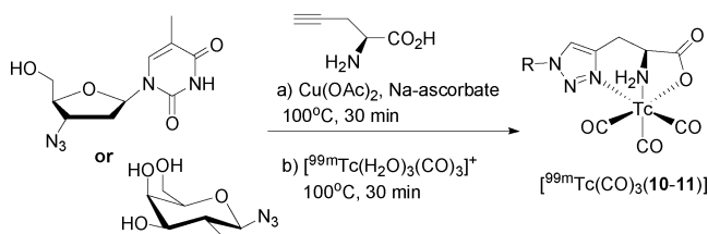
Scheme 2. One-Pot Procedure to Yield Radiolabeled Conjugates Directly
