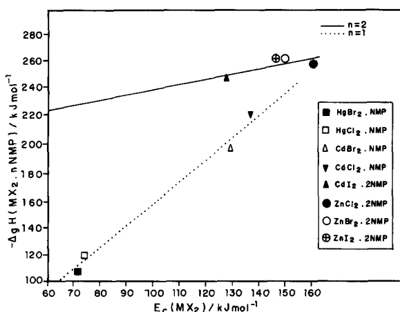
Fig. 4. \Delta_g H^0(MX_2 \cdot nNMP) values vs. covalent energy ( E_c ) of the metal halides.
