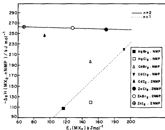
Fig. 3. \Delta_g H^0(MX_2 \cdot nNMP) values vs. ionic energy ( E_i ) of the metal halides.
