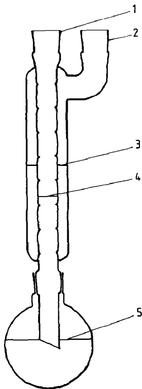
Fig. 1. The modified apparatus: 1,2 – ground joints, 3 – level of cooling liquid, 4 – level of the cooled part of the reaction mixture, 5 – level of the heated part of the reaction mixture.
