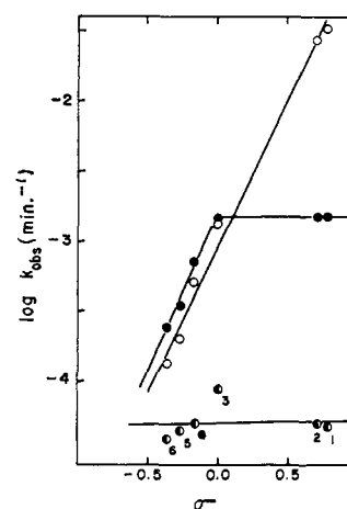
Figure 6. Dependence of the logarithm of k_{\text{obsd}} for the hydrolysis of six 2-arylthiazolines at three different pH values upon the substituent constants \sigma : \circ , pH 4.0; \bullet , pH 2.5; \circ , pH 0.5. Numbers refer to compounds of Figure 1.
