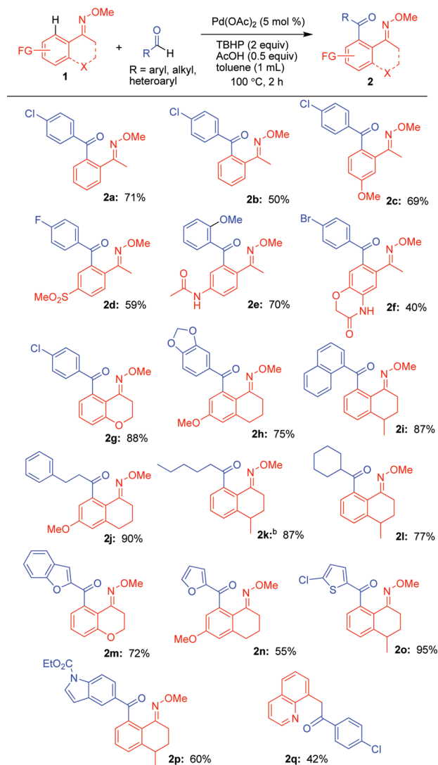
Scheme 1. Pd-Catalyzed Oxidative C–H Bond Coupling with Aldehydes a
