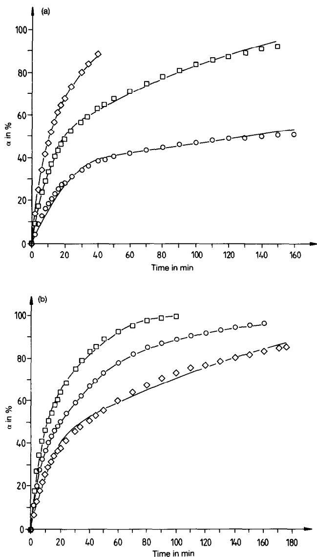
Fig. 5. Calculated and observed conversion vs. time curves. a. p = 10.1 \text{ kPa CCl}_4 : \circ , 620 K; \square , 680 K; \diamond , 750 K. b. T = 740 \text{ K} : \diamond , 2.5 kPa; \circ , 5.0 kPa; \square , 7.5 kPa \text{CCl}_4 .
