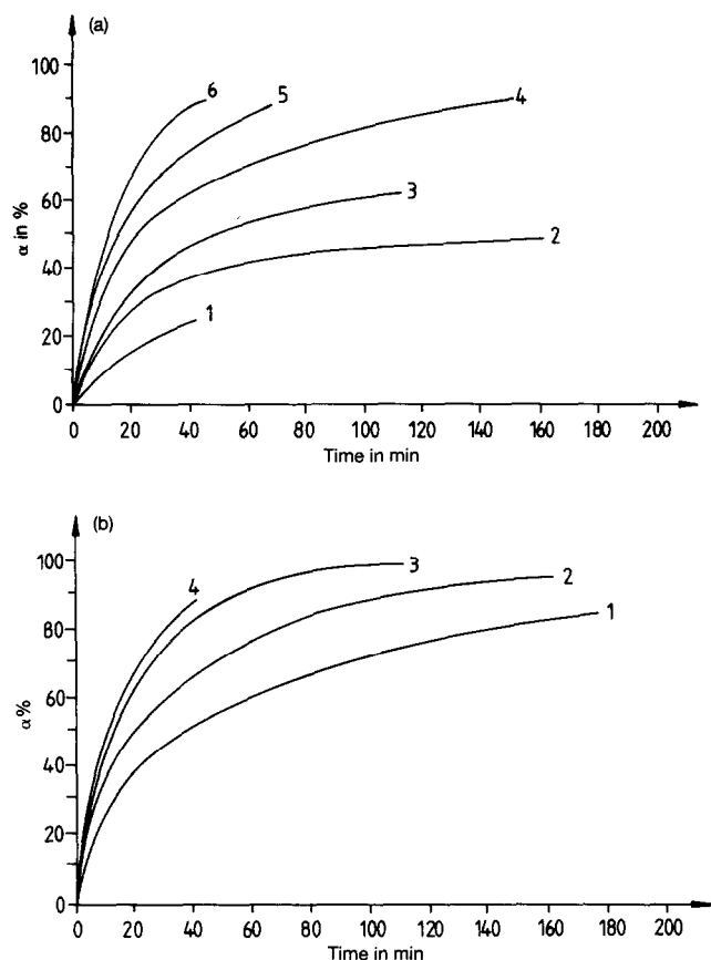
Fig. 1. Conversion versus time curves. a. p = 10.1 \text{ kPa CCl}_4 : curve 1, 580 K; curve 2, 620 K; curve 3, 650 K; curve 4, 680 K; curve 5, 700 K; curve 6, 740 K. b. T = 740 \text{ K} : curve 1, 2.5 kPa; curve 2, 5.0 kPa; curve 3, 7.6 kPa; curve 4, 10.1 kPa \text{CCl}_4 .
