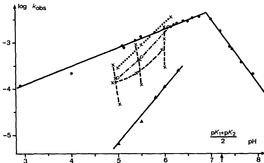
Fig. 1. Relationship between the logarithms of observed rate constants ( k_{\text{obs}} ) of the hydrolysis of 4-chloro-2-nitrobenzenediazonium tetrafluoroborate (4) and pH of buffer solutions ( I=0.50 ) at 30°.
