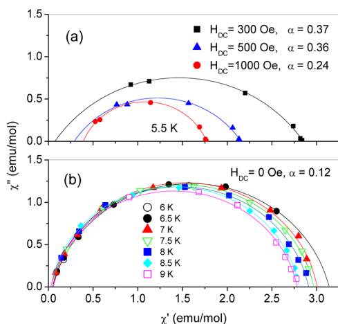
Figure 12. Comparison of Argand plots for meta -F compound obtained at 5.5 K in various dc magnetic fields (a) and for ortho -F obtained at various temperatures in 0 Oe dc field (b). The arcs are fits to the data.
