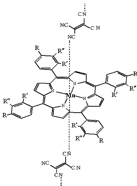
Figure 1. Molecular structure of Mn(III) tetra(phenyl)-porphyrin-tetracyanoethene. R, R', R'' labels denote para , ortho and meta positions of the phenyl ring, respectively.
