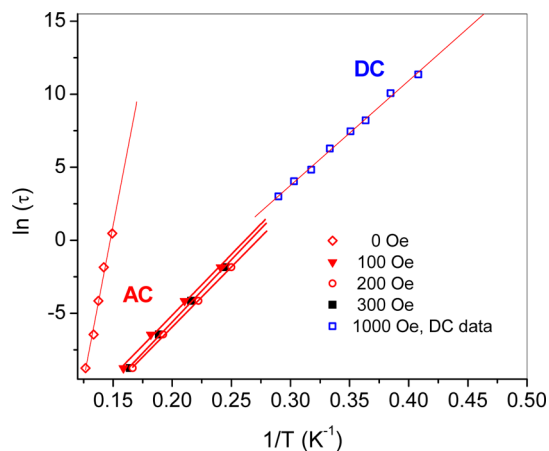
Figure 13. Natural logarithm of the relaxation time vs reciprocal temperature dependence for meta -F compound. The high temperature data (red color) were obtained from ac susceptibility measurements. The left (most steep) line was obtained in zero bias magnetic field, and the other three lines were obtained for nonzero bias magnetic fields. Dc data are also shown (see section 4.2.1). Solid lines are fits.
