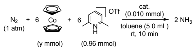
(a) Effect of CoCp 2 concentration
