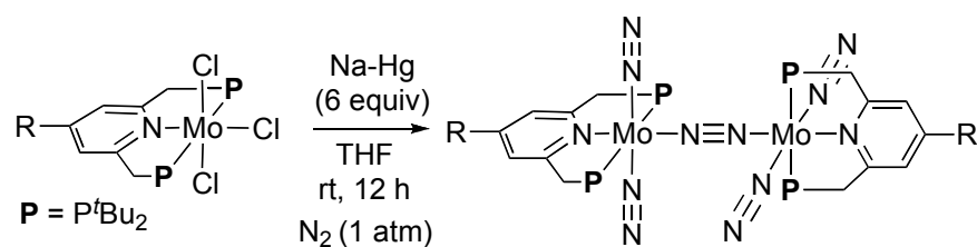
Scheme 2. Synthesis of Dinitrogen-Bridged Dimolybdenum-Dinitrogen Complexes Bearing 4-R-PNP-Pincer Ligands ( 1 ).
