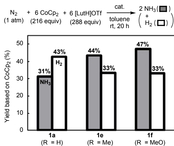
Figure 10. Yields of ammonia and molecular dihydrogen with 1a , 1e , and 1f as catalysts.
