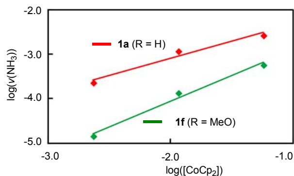
Figure 8. (a) Rate measurement for the formation of ammonia from molecular dinitrogen with 1a (red) and 1f (green) as catalysts at different initial CoCp 2 concentrations. (b) Plots of log(v(NH 3 )) against log([CoCp 2 ]).
