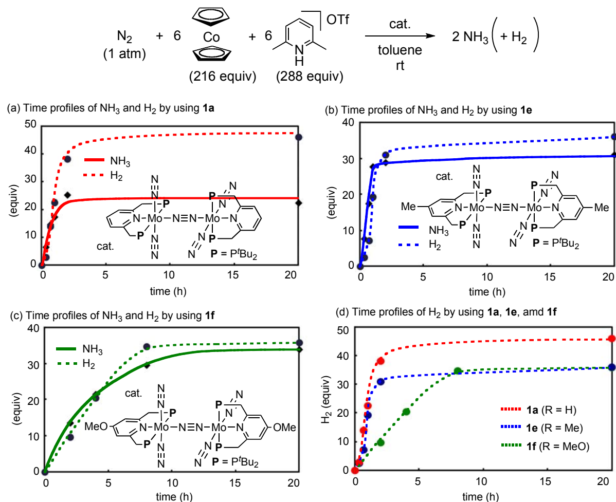
Figure 9. Time profile of the formation of ammonia (solid line) and molecular dihydrogen (dot line) with 1a (a), 1e (b), and 1f (c) as catalysts. (d) Time profiles of the formation of molecular dihydrogen with 1a , 1e , and 1f as catalysts.
