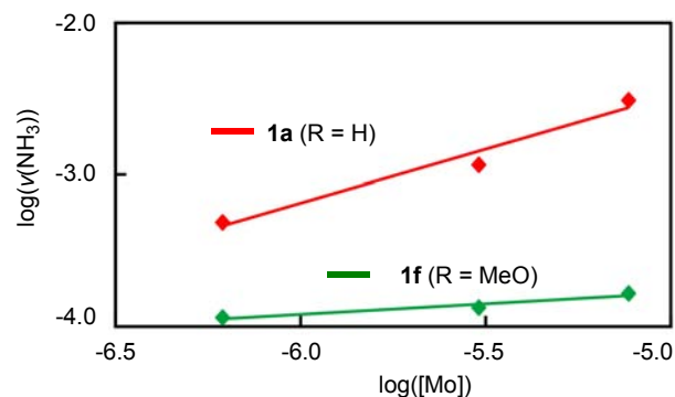
Figure 7. (a) Rate measurement for the formation of ammonia from molecular dinitrogen with 1a (red) and 1f (green) as catalysts at different initial Mo concentrations. (b) Plots of \log(v(\text{NH}_3)) against \log([\text{Mo}]) .
