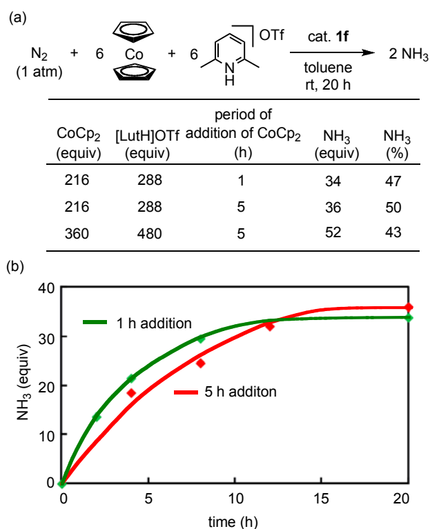
Figure 6. (a) Catalytic formation of ammonia from molecular dinitrogen using 1f as a catalyst.
