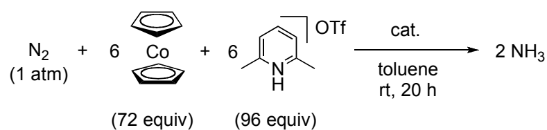
Scheme 3. Catalytic Formation of Ammonia Using Dimolybdenum-Dinitrogen Complexes Bearing Unsymmetric PNP-Pincer Ligand as Catalysts.
