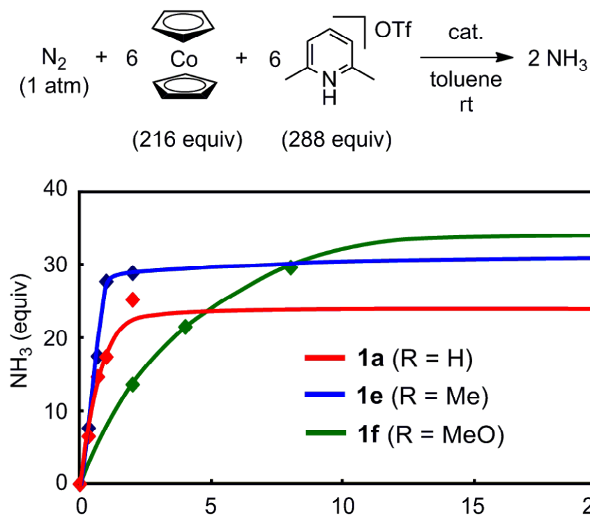
Figure 5. Time profiles of the formation of ammonia from molecular dinitrogen with 1a (red), 1e (blue), and 1f (green) as catalysts.
