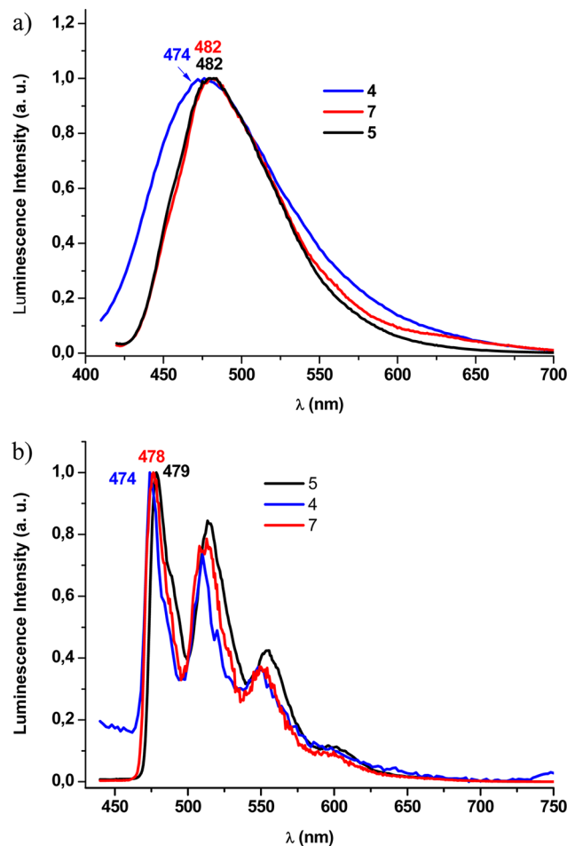
Figure 7. Normalized emission spectra of (a) 4 and (b) 5 in CH_2Cl_2 5 \times 10^{-4} M at 298 K and at 77 K.
