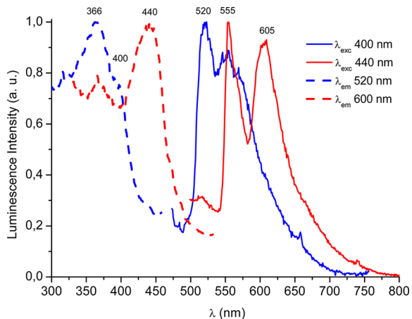
Figure 6. Normalized excitation and emission spectra of [Pt(bzq)-(C_6F_5)_2(\eta^2-PhC \equiv CPh)] ( 7 ) in solid state at 77 K.
