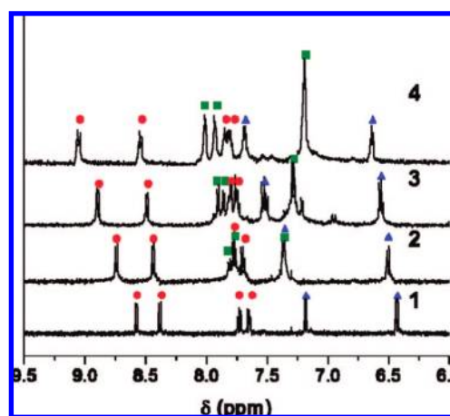
Figure 2. ^1\text{H} NMR spectra of the aromatic regions of 1–4 at 300 K in \text{CDCl}_3 . Red circles denote peaks from CA, blue triangles denote peaks from PP, and green squares denote peaks from the bridge. Notice the downshifting CA peaks.
