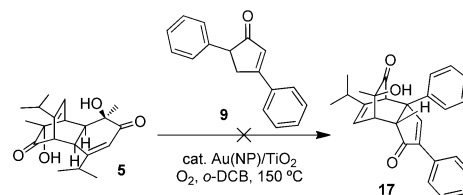
Scheme 4. In Situ Trapping Experiment
