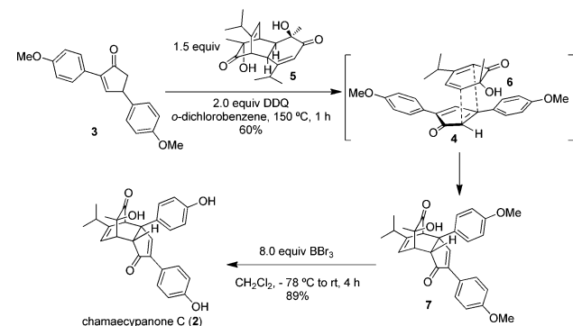
Scheme 2. First-Generation Synthesis of Chamaecyanone C
