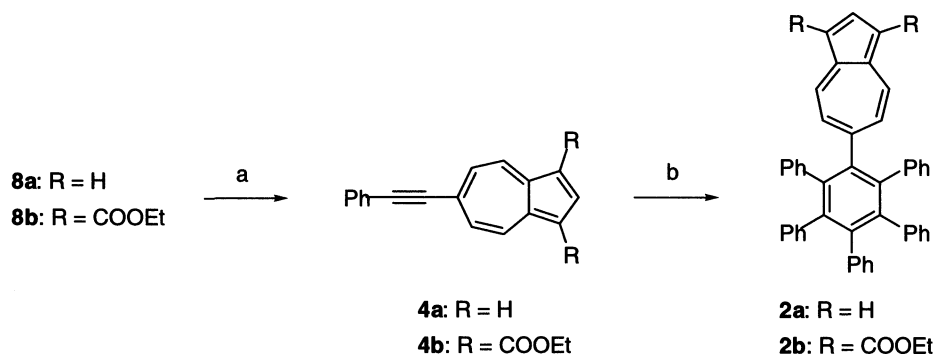
Scheme 3. Synthesis of 2a and 2b . (a) Phenylacetylene, [\text{PdCl}_2(\text{PPh}_3)_2] , \text{PPh}_3 , \text{CuI} , \text{Et}_3\text{N} , toluene, rt, 5 h (90%) for R = H, 9 h (87%) for R = COOEt; (b) 5 , diphenyl ether, 160^\circ\text{C} , 1 day (32%) for R = H, 140^\circ\text{C} , 5 days (93%) for R = COOEt
