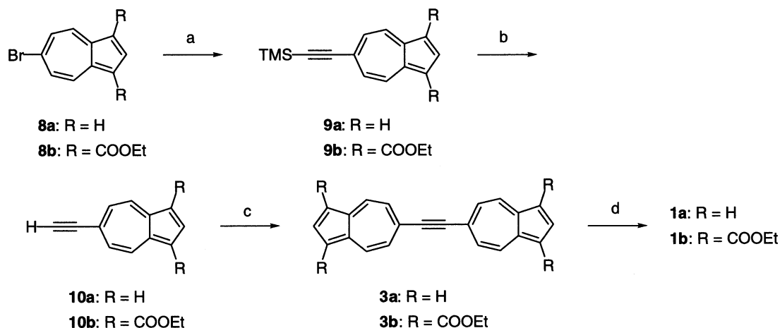
Scheme 2. Synthesis of 1a and 1b . (a) TMSA, [\text{PdCl}_2(\text{PPh}_3)_2] , \text{PPh}_3 , \text{CuI} , \text{Et}_3\text{N} , toluene, rt, 2.5 h (86%) for R = H, 1.5 h (84%) for R = COOEt; (b) \text{KF} , \text{H}_2\text{O} , DMF, rt, 3 h (78%) for R = H, 3 h (93%) for R = COOEt; (c) 8a and 8b , [\text{Pd}(\text{PPh}_3)_4] , \text{PPh}_3 , \text{CuI} , \text{Et}_3\text{N} , toluene, rt, 3 h (98%) for R = H, 1.5 h (96%) for R = COOEt; (d) 5 , diphenyl ether, 160^\circ\text{C} , 2 days (13%) for R = H, 1 day (91%) for R = COOEt
