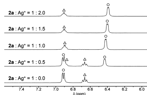
Figure 2. \text{Ag}^+ -ion-induced ^1\text{H} NMR shift changes of 2a (aromatic region) in a mixture of \text{CD}_2\text{Cl}_2 and \text{CD}_3\text{OD} (0.75 mL/0.02 mL). As the intensities of the doublet at \delta 6.4 ppm and the triplet at \delta 6.9 ppm increase, the intensities of the doublet at \delta 6.6 ppm and the triplet at \delta 6.65 ppm decrease. The exchange rate of the complex and the metal-free ligand would be slower than the NMR time scale under the conditions used because the cyclen units bind \text{Ag}^+ ions strongly.
