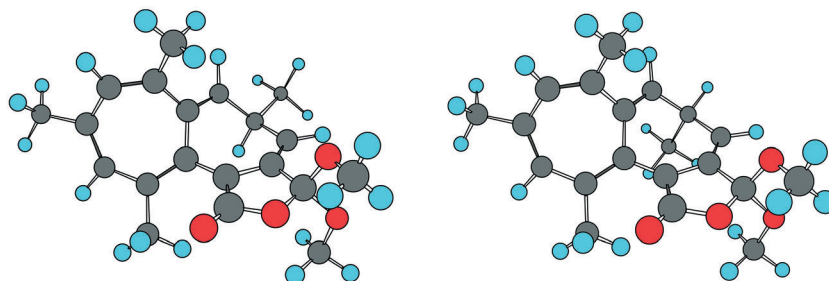
Fig. 7. AM1-Calculated, hypothetical dienolate structures resulting from re (left) and si (right) attack, resp., of methanide at C(5) of ( P )-configured furanone 28 (see text)
