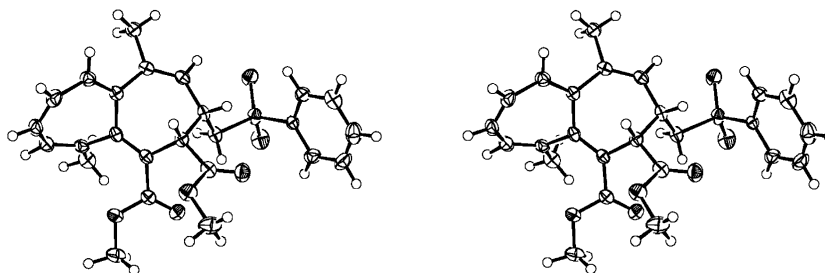
Fig. 3. Stereoscopic view of the X-ray crystal structure of dimethyl ( P^* , 3S^* , 4S^* )-3,4-dihydro-1,6-dimethyl-3-[(phenylsulfonyl)methyl]heptalene-4,5-dicarboxylate (( P^* )- 10 ; 50% probability ellipsoids)
