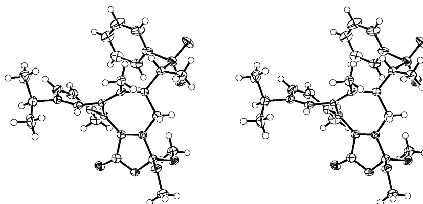
Fig. 5. Stereoscopic view of the X-ray crystal structure of one of the two symmetry-independent molecules of (P*,5 S *)-4,5-dihydro-8-isopropyl-3,3-dimethoxy-5-[(1 R *)-1-(phenylsulfonyl)ethyl]heptaleno[1,2- c ]-furan-1(3 H )-one ((P*)- 27 ; 50% probability ellipsoids)
