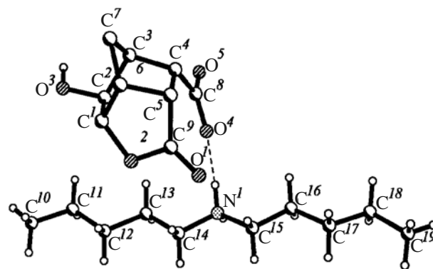
Fig. 2. Molecular structure of dipentylammonium exo -2-hydroxy-5-oxo-4-oxatricyclo[4.2.1.0 3,7 ]nonane- endo -9-carboxylate ( XVI ) according to X-ray diffraction analysis
