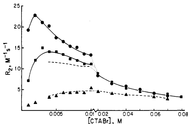
Figure 2. Variation of second-order rates with [CTABr] in 0.005 M NaCN: \blacklozenge , \blacksquare , \bullet , R = C_{12}H_{25} , C_{14}H_{29} , and C_{16}H_{33} , respectively. The broken lines are calculated.
