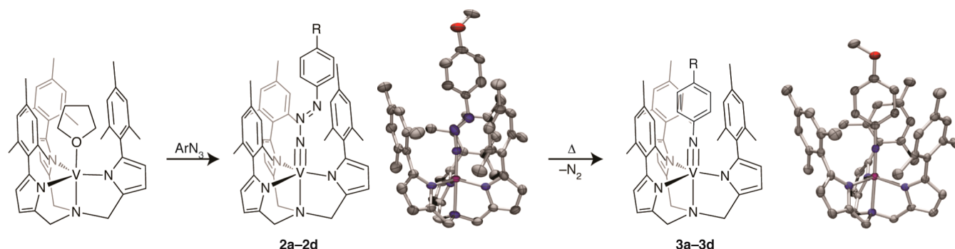
Figure 1. Synthetic scheme for the formation of vanadium(V) diazenylimido and vanadium(V) imido species supported by the tripyrrolyl ligand \text{tpa}^{\text{Mes}} ; R = OMe (a); H (b); OMe (c), \text{NMe}_2 (d). ORTEP crystal structures for 2a and 3a with thermal ellipsoids drawn at 50% probability, with solvent molecules and hydrogen atoms omitted for clarity, are also shown.
