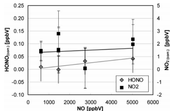
Figure 5. HONO and \text{NO}_2 mixing ratios in the reaction \text{HNO}_3 + NO corrected for the blank signals of pure NO as a function of the NO mixing ratio. ( [\text{HNO}_3] = 750 ppbV, RH = 30%, T = 298 \pm 1 K).
