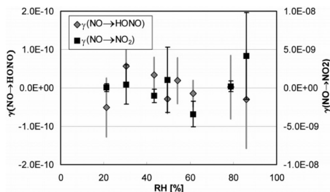
Figure 6. Reactive uptake coefficients γ(NO→HONO) and γ(NO→NO 2 ) as a function of relative humidity. The errors bars represent the statistical precision (2σ) of the linear least-squares fits as shown in Figure 5. (HNO 3 mixing ratio = 350–750 ppbV, T = 300 ± 3 K).
