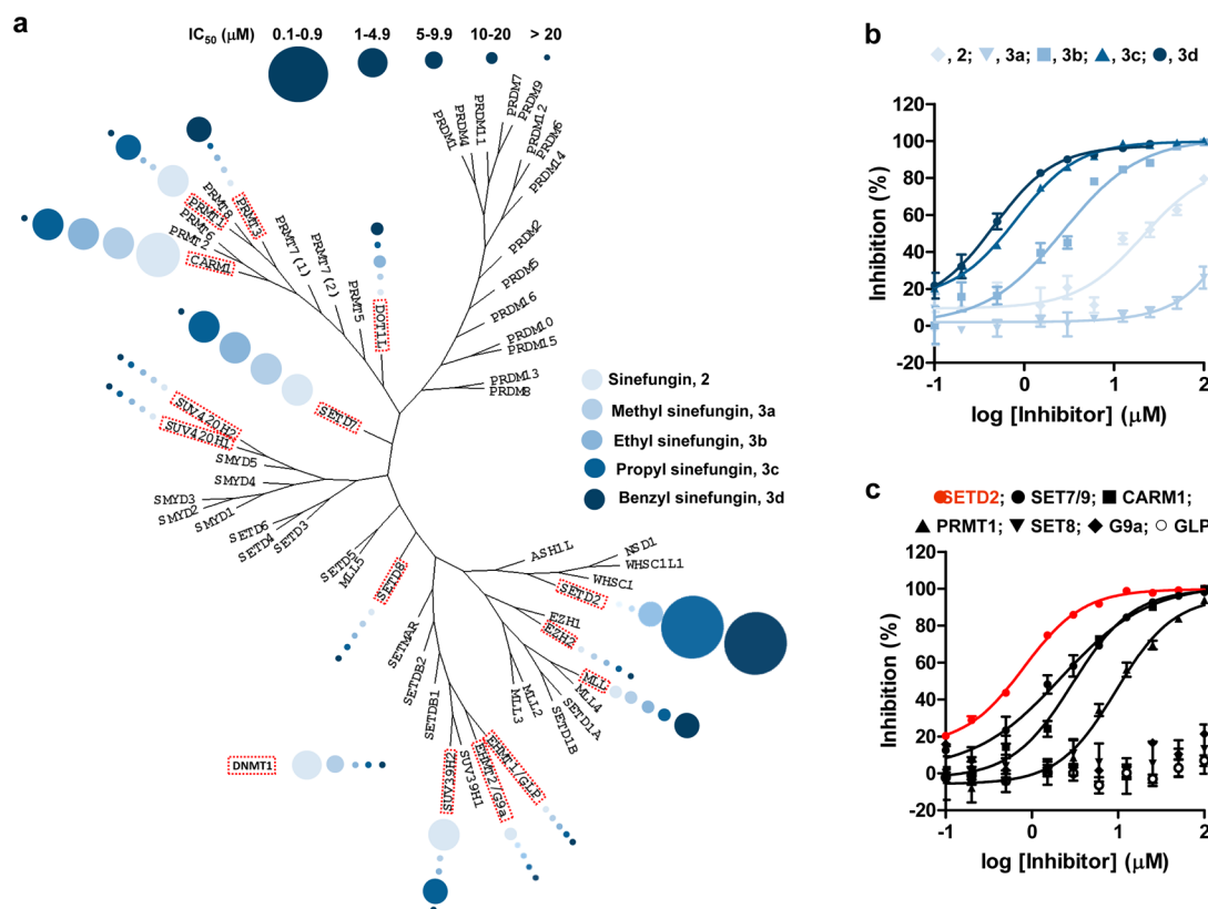
Figure 2. Inhibition profile of sinefungin and its analogues 3a–d against a panel of methyltransferases. (a) The magnitude of IC_{50} of sinefungin and its analogues 3a–d is presented against 15 phylogenetically arrayed methyltransferases (their IC_{50} values are listed in Table S1). The increased diameters and darkness of the circles reflect higher potency (lower IC_{50} ) and larger sizes of the inhibitors, respectively. (b) Representative IC_{50} curves of sinefungin and its analogues 3a–d against SETD2 with the values of 28.4 \pm 1.5 , >100 , 8.2 \pm 1.2 , 0.80 \pm 0.02 , and 0.48 \pm 0.06 \mu M for sinefungin and 3a–d , respectively. (c) IC_{50} curves of Pr-SNF 3c against representative methyltransferases with the values of 0.80 \pm 0.02 \mu M for SETD2, 2.2 \pm 0.4 \mu M for SET7/9, 3.0 \pm 0.3 \mu M for CARM1, 9.5 \pm 0.4 \mu M for PRMT1, >100 \mu M for SET8, G9a, and GLP.
