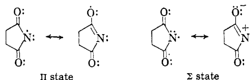
Figure 1. Representative \Pi and \Sigma Lewis electronic structures for the succinimidyl radical.
