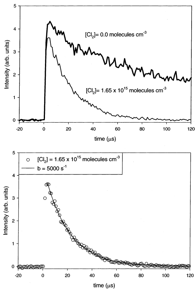
Figure 3. Representative H + Cl 2 data are shown. The slow decay in the absence of Cl 2 in the upper panel is attributed mainly to diffusion out of the observation zone with a minor amount of H atom loss via reactions with photoproducts. The lower panel demonstrates the quality of the fit to a single-exponential decay. The corresponding decay rate is 5000 s -1 .
