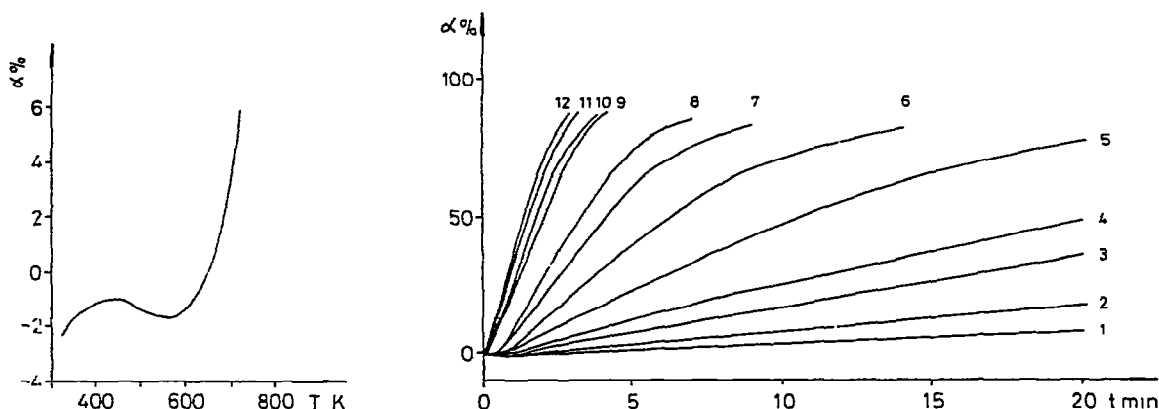
Fig 1 Anisothermal TG curve of the reaction of \gamma\text{-Al}_2\text{O}_3 with \text{CO} + \text{Cl}_2 mixture. Linear heating rate = 5\text{ K min}^{-1} , P_{\text{CO}} = P_{\text{Cl}_2} = 5 \times 10^4\text{ Pa}
