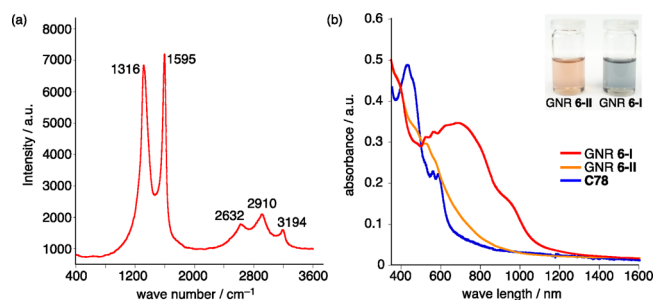
Figure 5. (a) Raman spectrum of GNR 6-I measured at 488 nm (powder, laser power: 1 mW). (b) Normalized UV–vis absorption spectra of GNR 6-I (red, in NMP), GNR 6-II (orange, in NMP), and C78 (blue, in THF); inset: a picture of solutions of GNR 6-I and 6-II in NMP.
