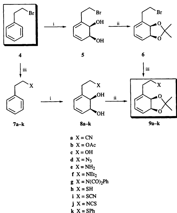
Scheme 1 Reagents and conditions: i, ( 7e–h not substrates) JM 109 ( E. coli ); ii, DMP, p TSA, CH 2 Cl 2 , room temp.; iii, (preparation of 7d , f , g , i , k , 9a , b , d , f–i , k ), Nu − , DMF, room temp.; (preparation of 9c ) NaOAc, DMF, room temp.; LAH, THF; (preparation of 9e ) NaN 3 , DMF, room temp.; PPh 3 , THF, H 2 O; compound 9j could not be obtained via nucleophilic substitution
