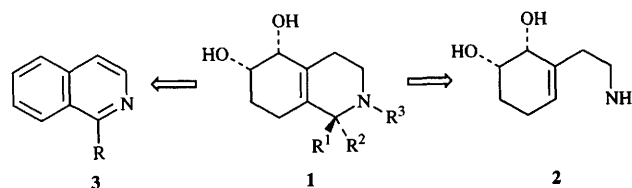
Fig. 1 Biocatalytic design of the synthesis of cis -5,6-dihydroxy-1,2,3,4,5,6,7,8-octahydroisoquinoline 1
