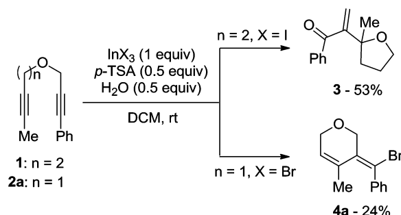
Scheme 1. Divergent Cyclization Catalyzed by In(III)
