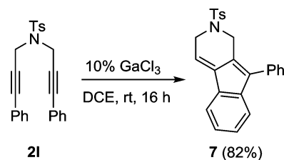
Scheme 2. Diphenyldiyne Cycloisomerization
